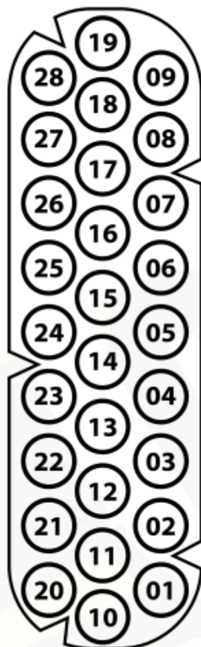
SENSOR CONNECTOR A
